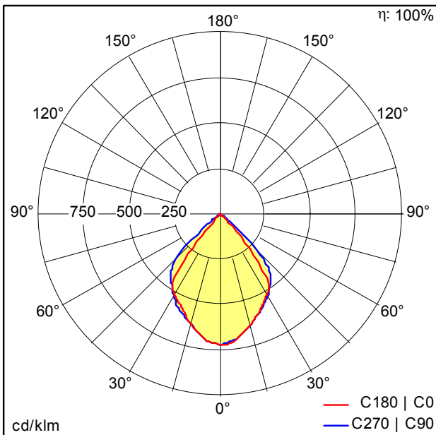
TE_HOLLY_CONE_DOWN_IP65_300_830.idt
